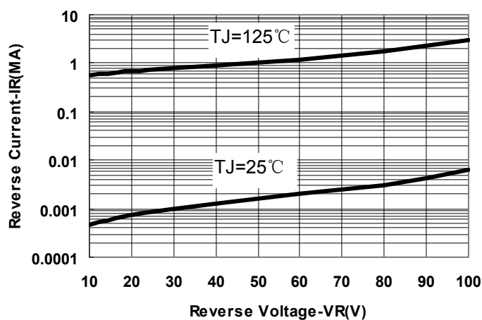
Fig.2-Typical Reverse Characteristics
