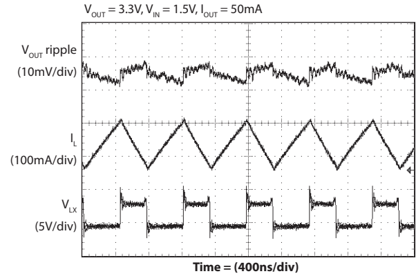
PWM Operation
