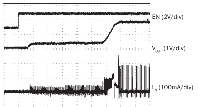
PSAVE Start-up
