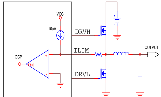
Figure 8. Block diagram of over current protection.
