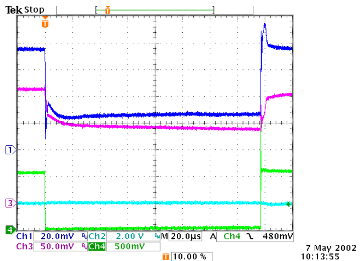
Load Transient Response, With Passive Droop
