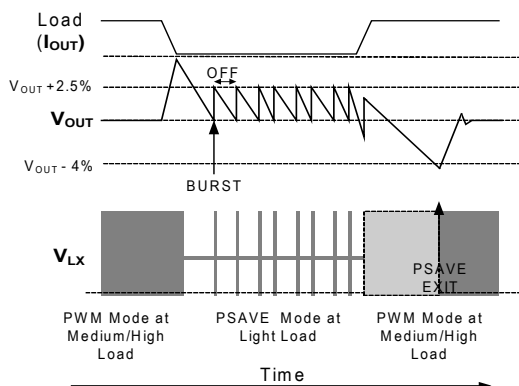
Figure 2 - Transitions Between PWM and PSAVE Modes
