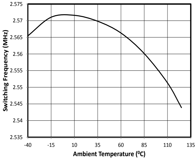
Switching Frequency Vs Temperature, V_{out}=1.5\text{V}
