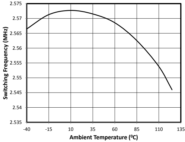
Switching Frequency Vs Temperature, V_{out}=1.0\text{V}
