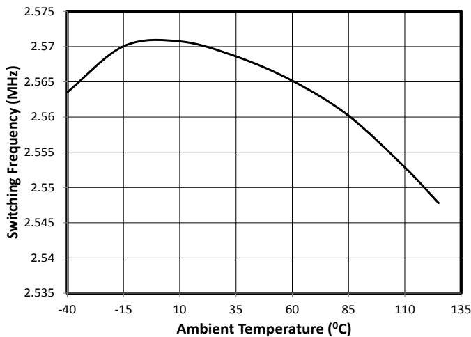
Switching Frequency Vs Temperature, V_{out}=2.5\text{V}
