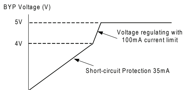
Figure 9 — LDO Start-Up
