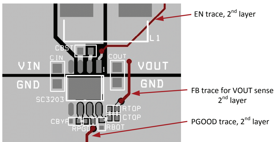
Figure 12 — PCB Layout
