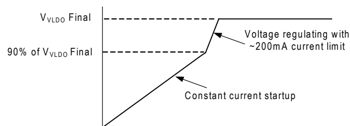
Figure 12 — LDO Start-Up
