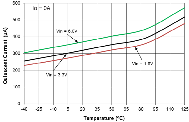
Quiescent Current
