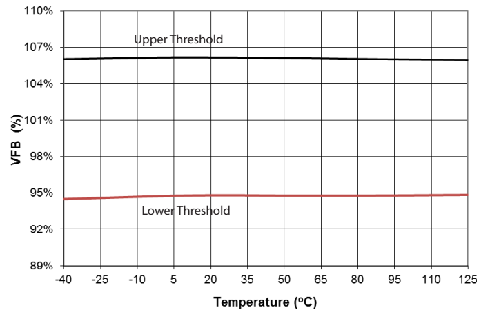
PG Threshold
