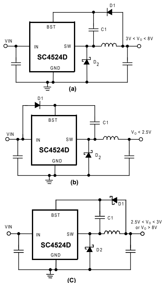
Figure 6 — Methods of Bootstrapping the SC4524D
