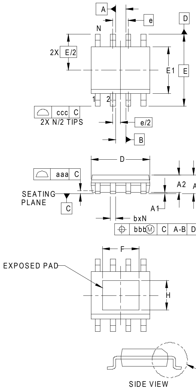
DETAIL A SEE DETAIL A
