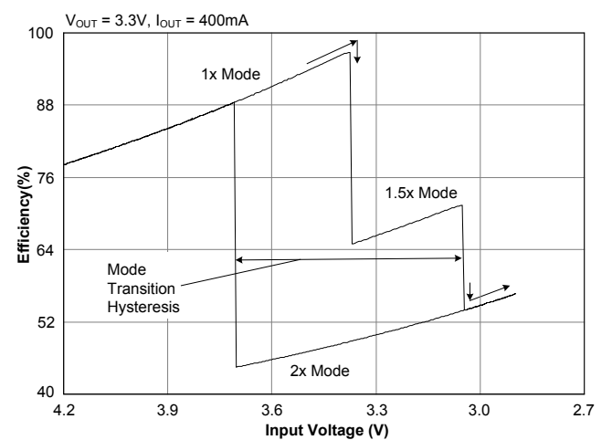
Efficiency — 400mA
