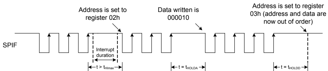
Figure 7 — Faulty SemPulse Data Write Due to Extended Interrupt Duration
