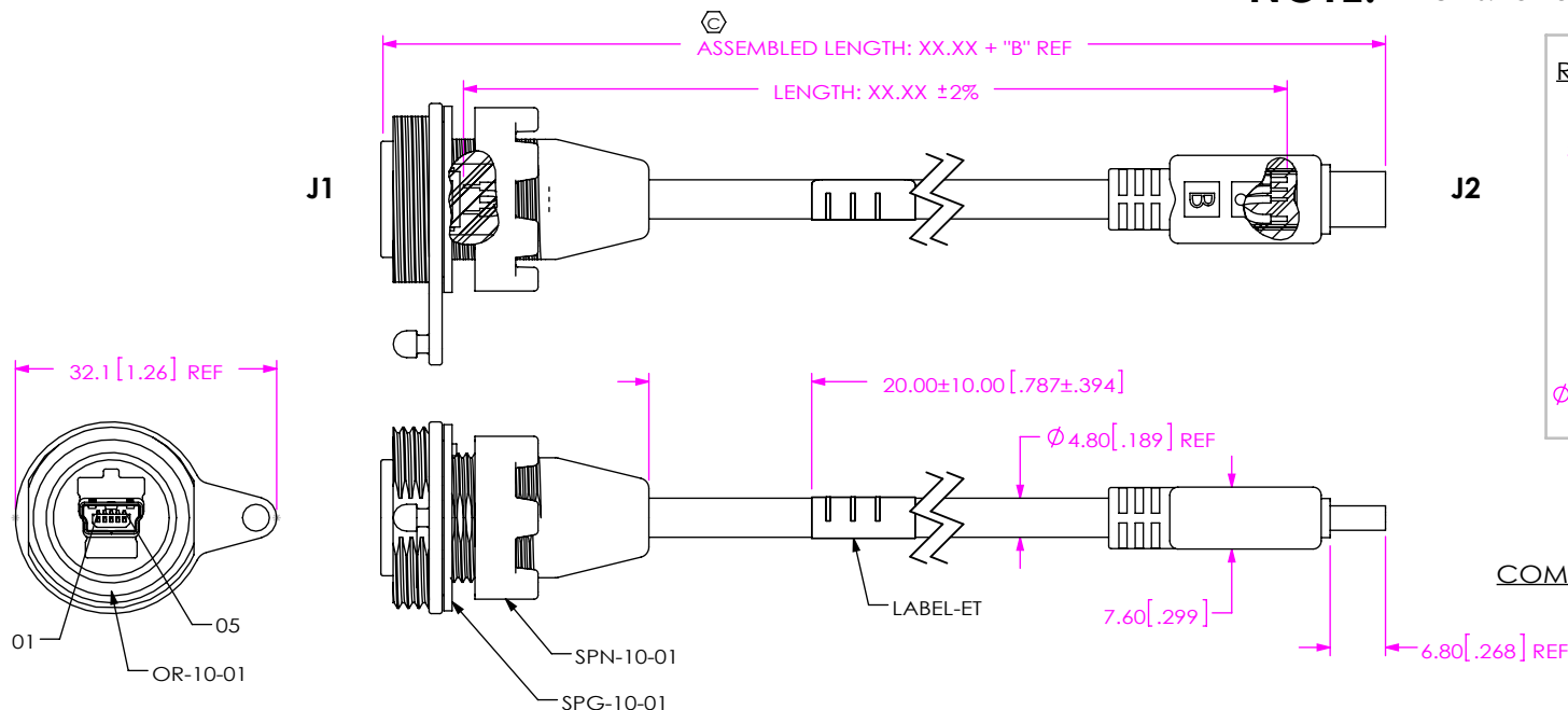
FIG 1 SCRUS-10-X-XX.XX-MBS-MB SHOWN
