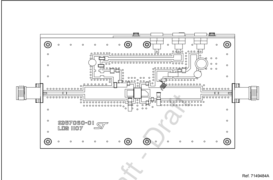
Figure 13. Test fixture
