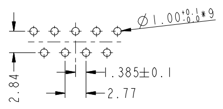
9 Pin Female Connector PCB Pin Layout Scale 2:1
