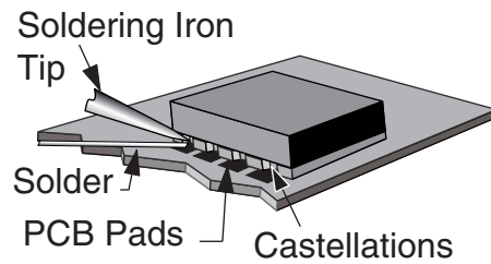
Figure 15: Soldering Technique
