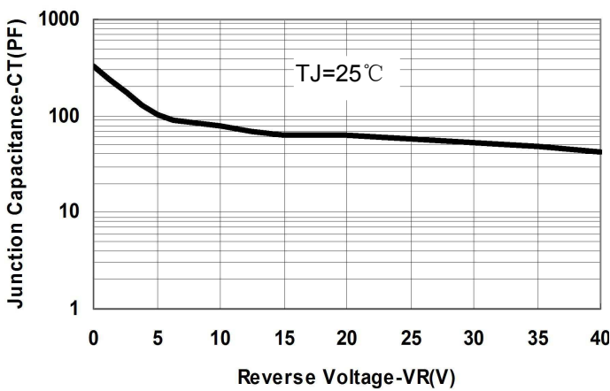
Fig.1-Typical Junction Capacitance
