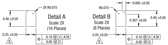
Figure 13. SE2435L Package Dimensions
