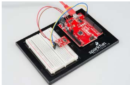
A SHT15 connected to the SDA(A4) and SCL(A5) lines on a SparkFun
