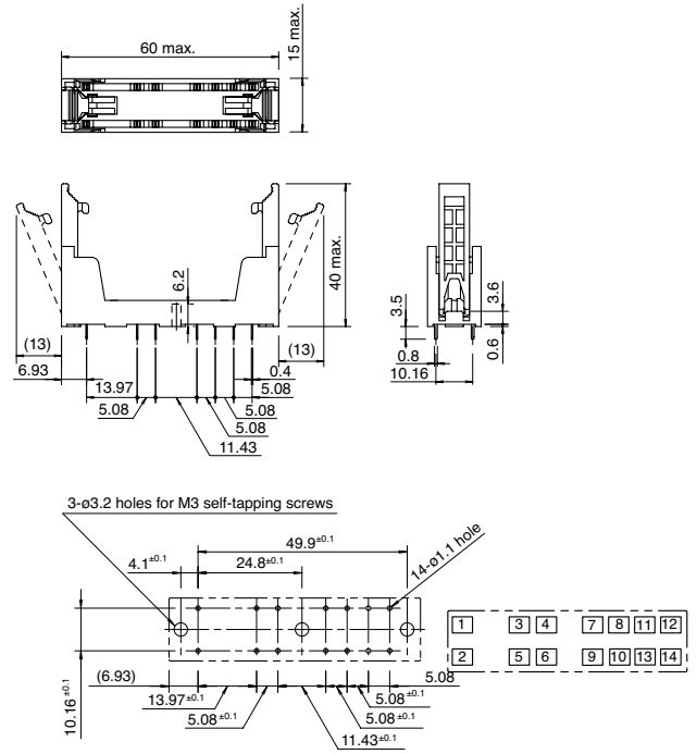
SF1V-6-07L (6-pole)
