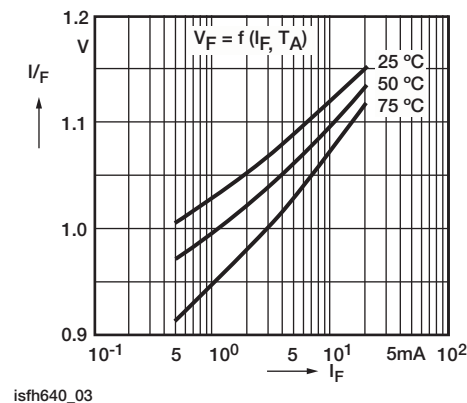
Fig. 4 - Diode Forward Voltage (typ.)
