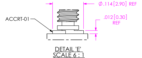
FIG 8 -DS: DUAL SCREW DOWN (SAME AS FIG 2, DIFFERENT AS SHOWN)
