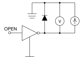
Figure 8 V_F Test Circuit
