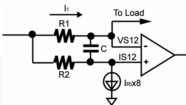
Figure 4. OCP Set-up
