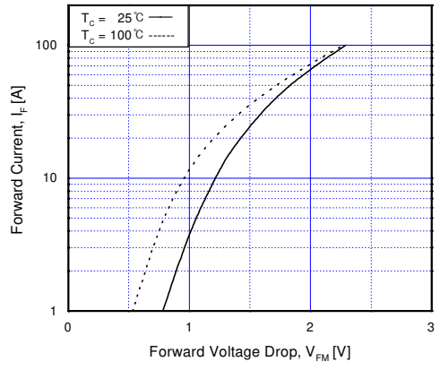
Fig 18. Forward Characteristics
