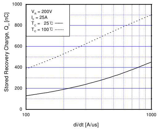
Fig 20. Stored Charge
