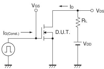
Fig.2-1 Gate Charge Measurement Circuit
