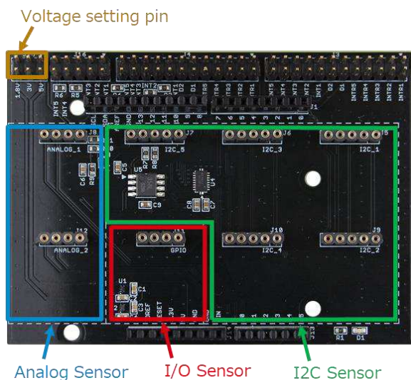
Figure 4. Voltage settings and Connection of the Sensors
