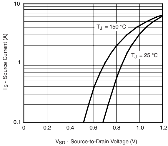
V_{SD} - Source-to-Drain Voltage (V) Forward Diode Voltage
