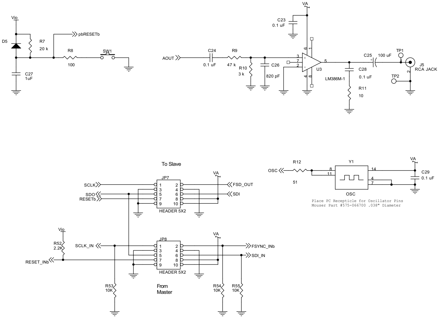
Figure 12. Si30xx Motherboard Schematic (2 of 2)
