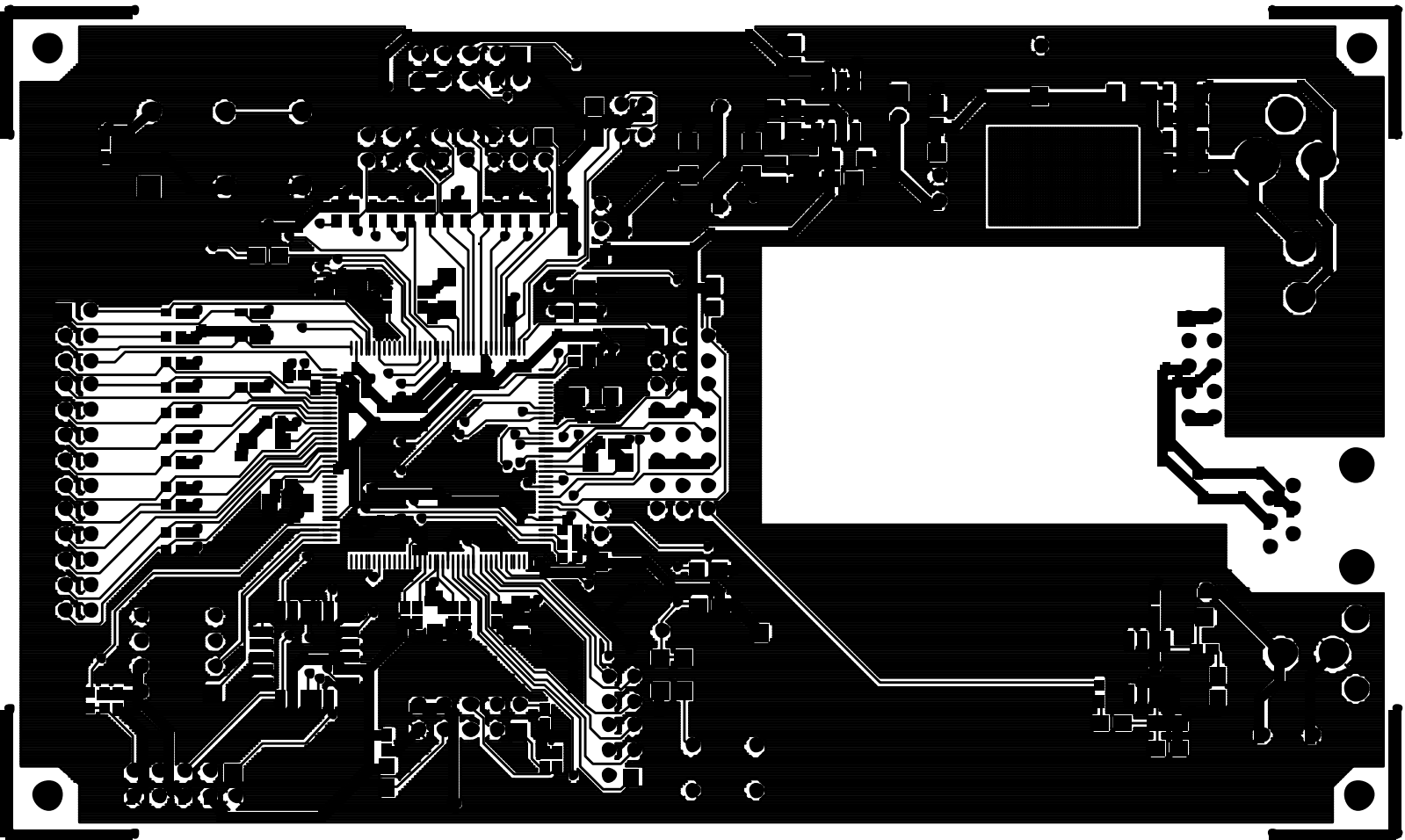
Figure 15. Si30xx Motherboard Component Layer
