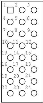
Footprint of JP1 Top View
