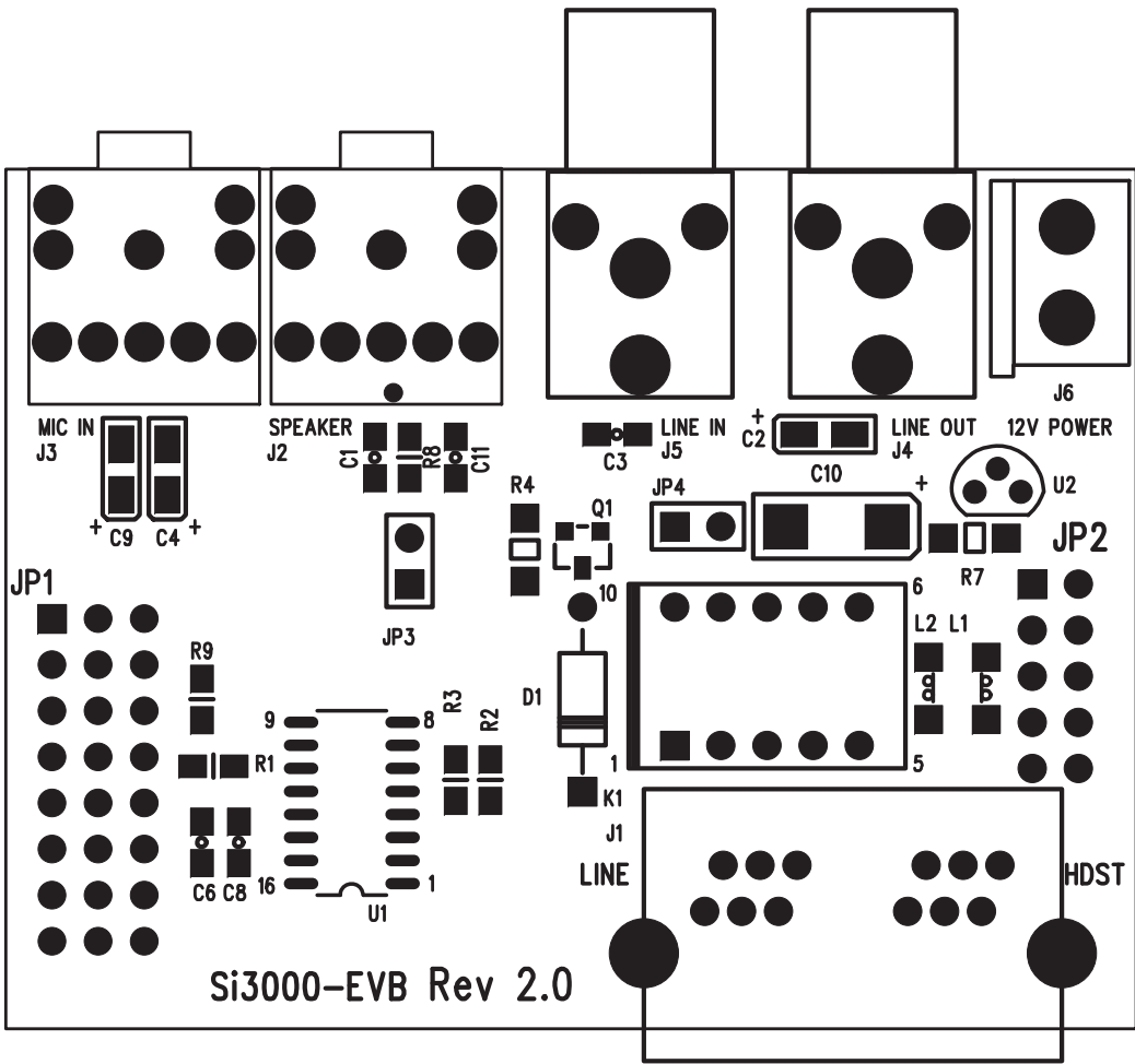
Figure 8. Si3000DC-EVB Silkscreen
