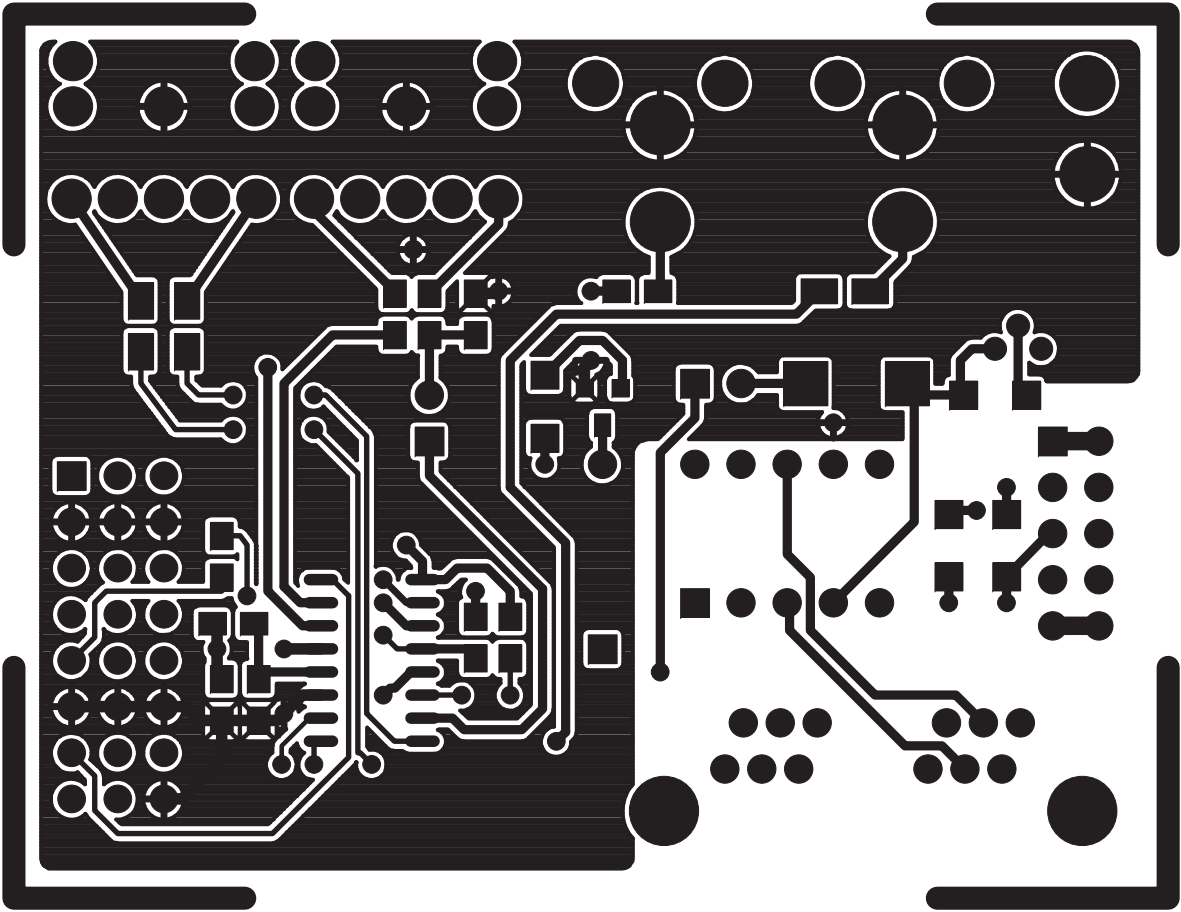
Figure 9. Si3000DC-EVB Component Side
