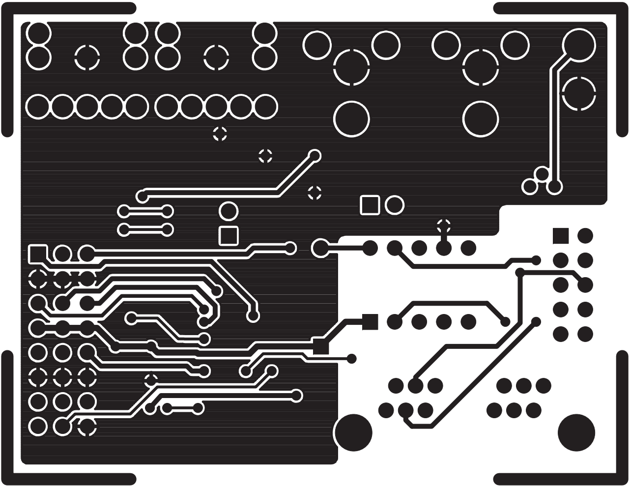
Figure 10. Si3000DC-EVB Solder Side
