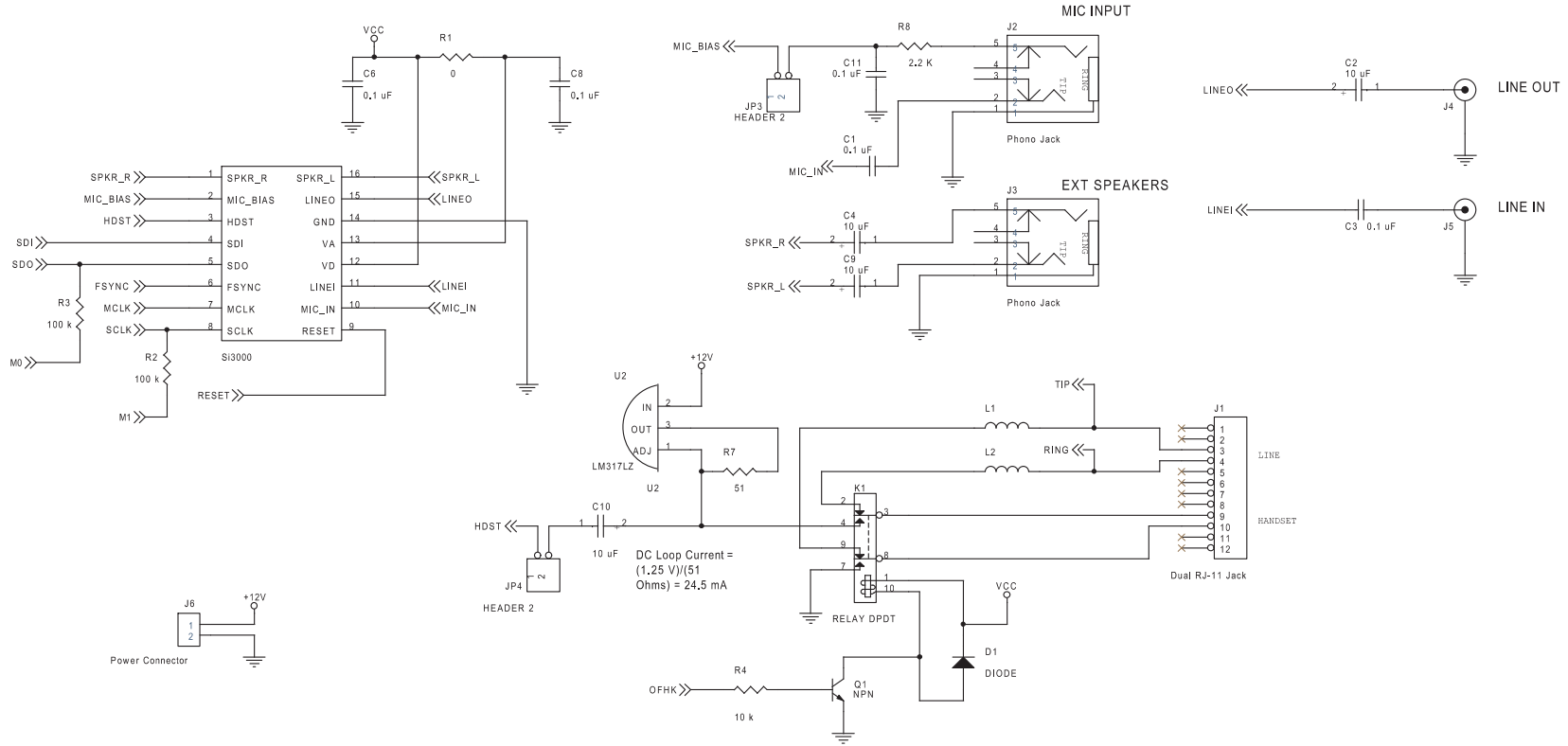
Figure 6. Si3000DC-EVB Schematic (1 of 2)
