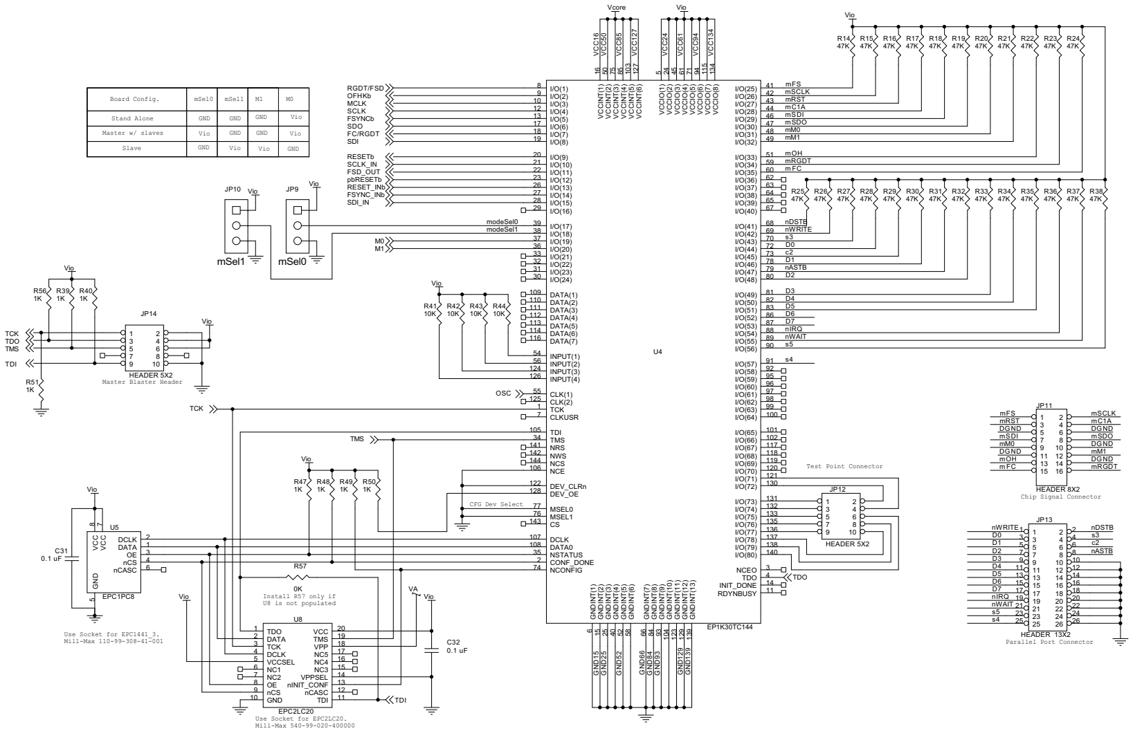
Figure 13. Si30xx Motherboard Schematic (3 of 3)
