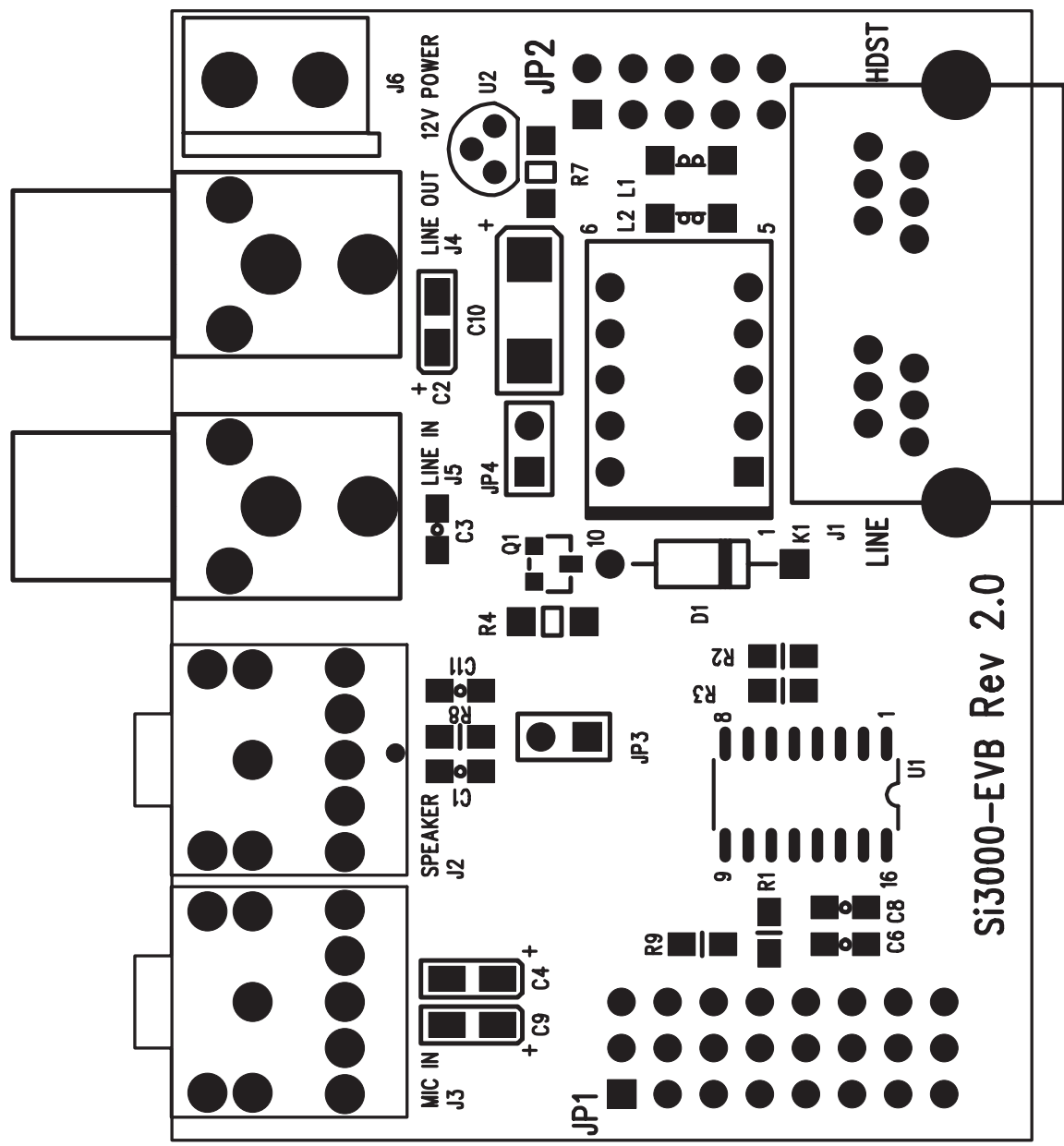
Figure 5. Si3000DC-EVB Silkscreen
