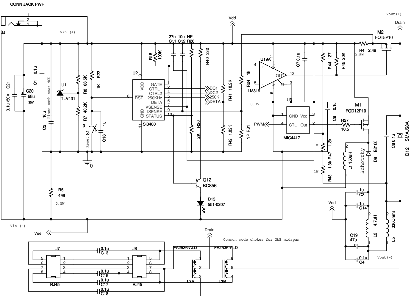
Figure 10. Si3460 and Power Circuit
