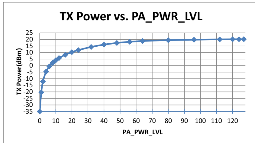
Figure 8. +20 dBm TX Power vs. PA_PWR_LVL
