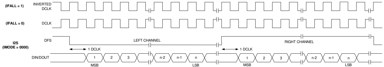
Figure 15. I 2 S Digital Audio Format
