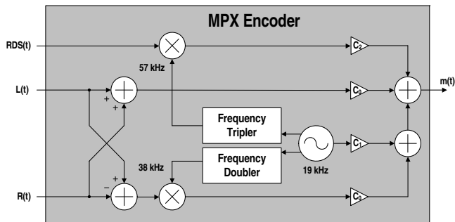
Figure 14. MPX Encoder
