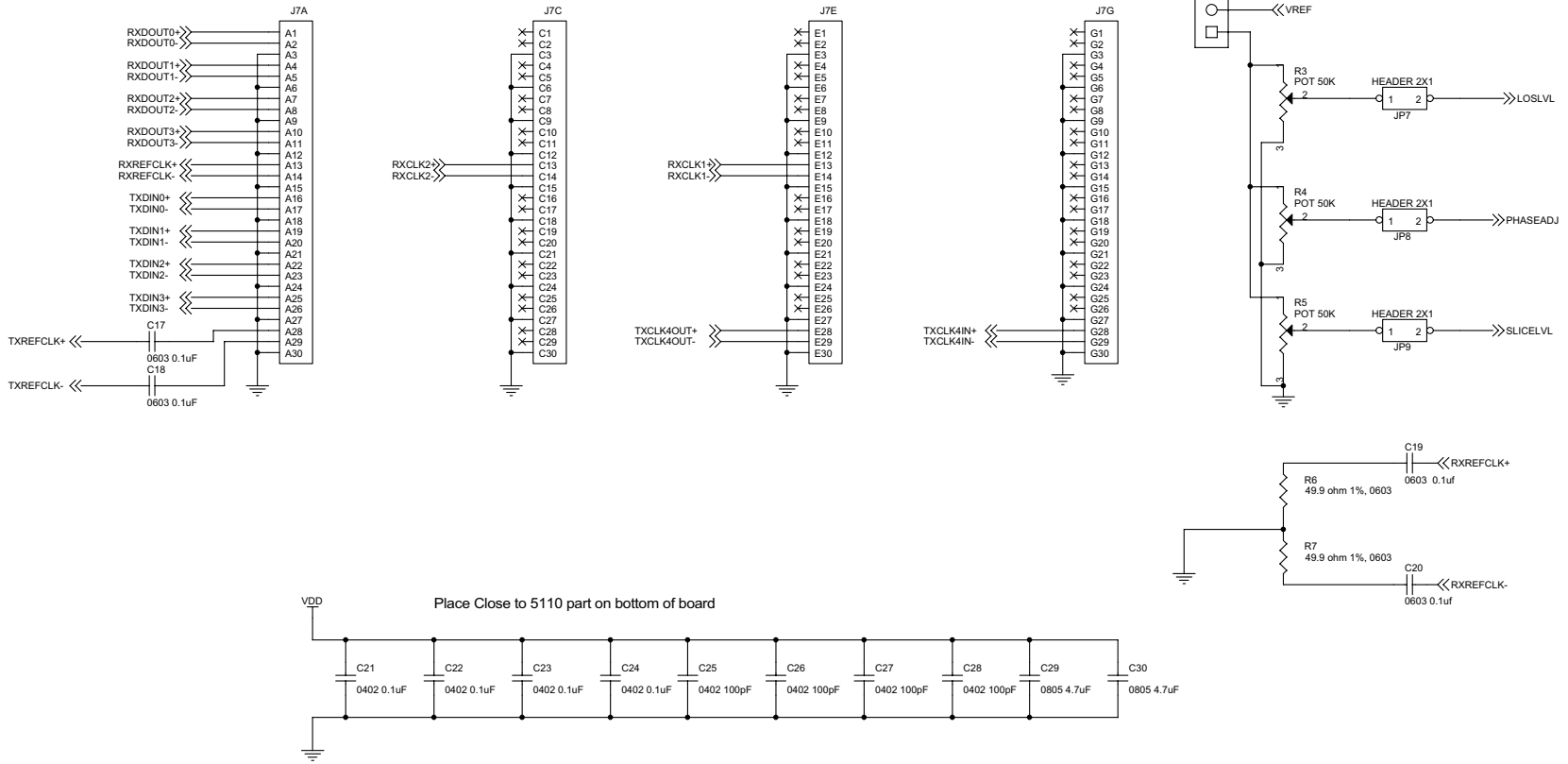
Figure 13. Si5110-EVB Daughter Card Schematic (page 3 of 3)
