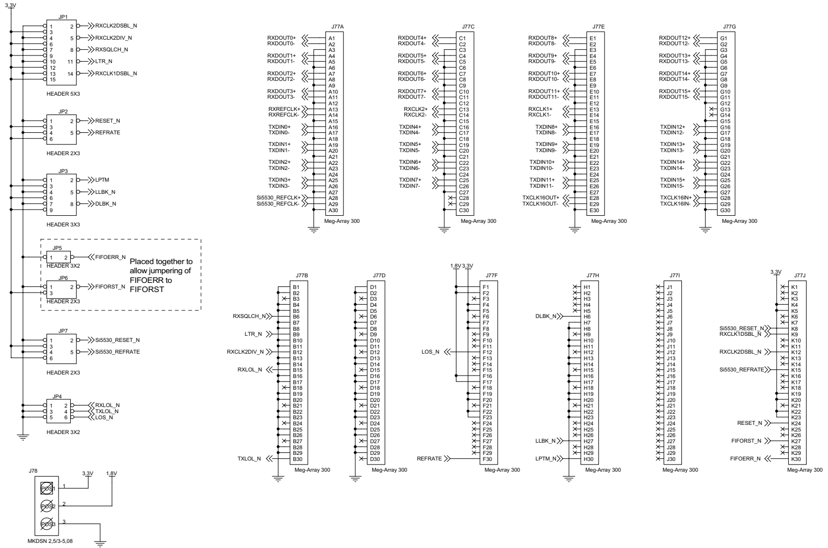
Figure 17. Full-Duplex Motherboard Schematic (page 2 of 2)
