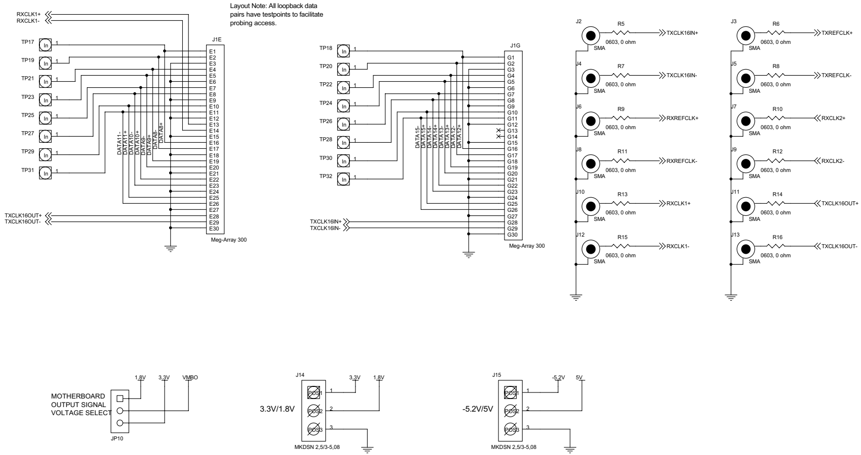
Figure 14. Loopback Motherboard Schematic (page 1 of 2)
