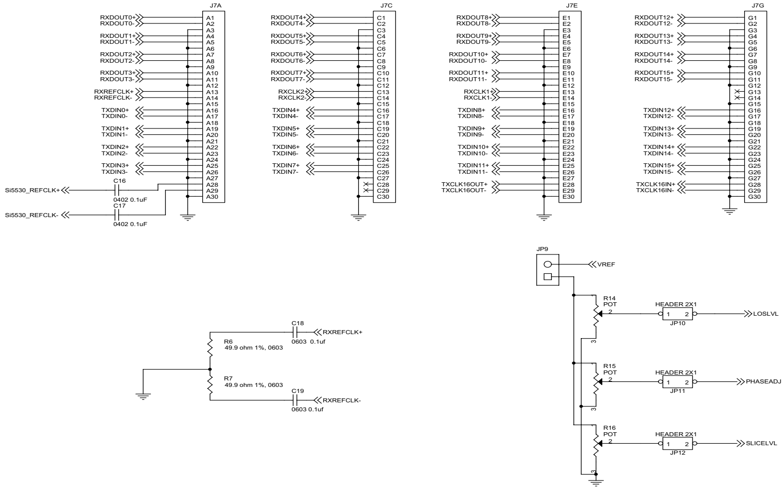
Figure 10. Si5100-EVB Daughter Card Schematic (page 3 of 3)
