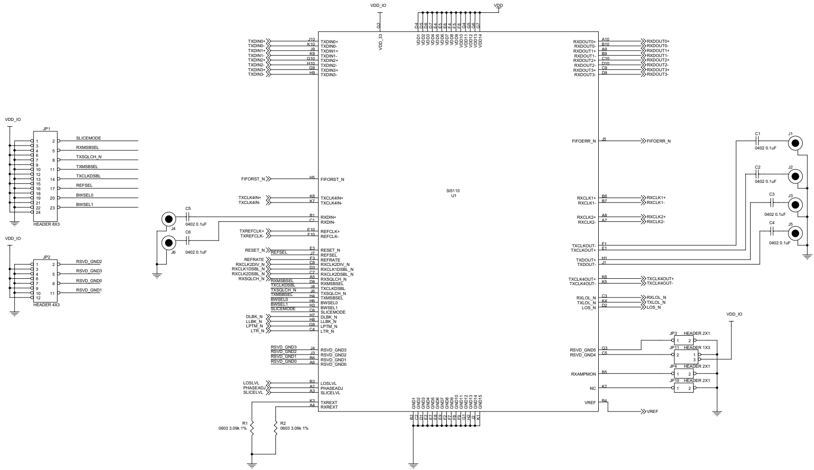
Figure 11. Si5110-EVB Daughter Card Schematic (page 1 of 3)
