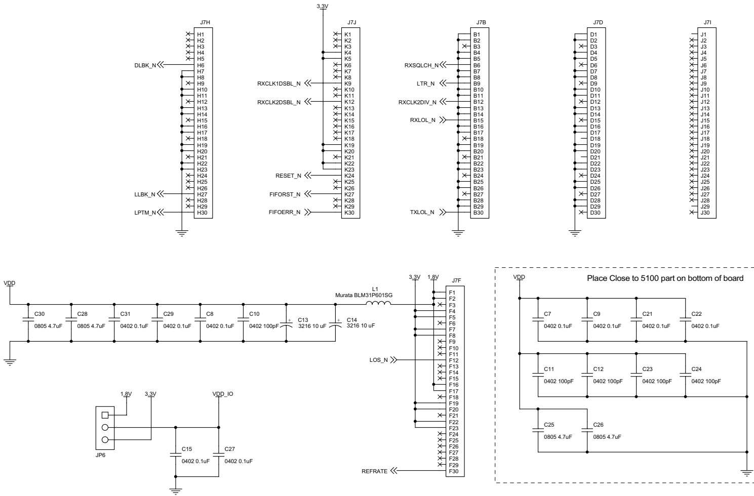
Figure 9. Si5100-EVB Daughter Card Schematic (page 2 of 3)
