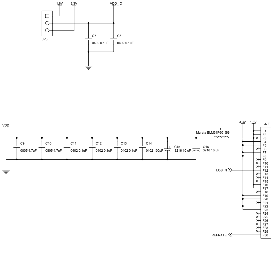
Figure 12. Si5110-EVB Daughter Card Schematic (page 2 of 3)
