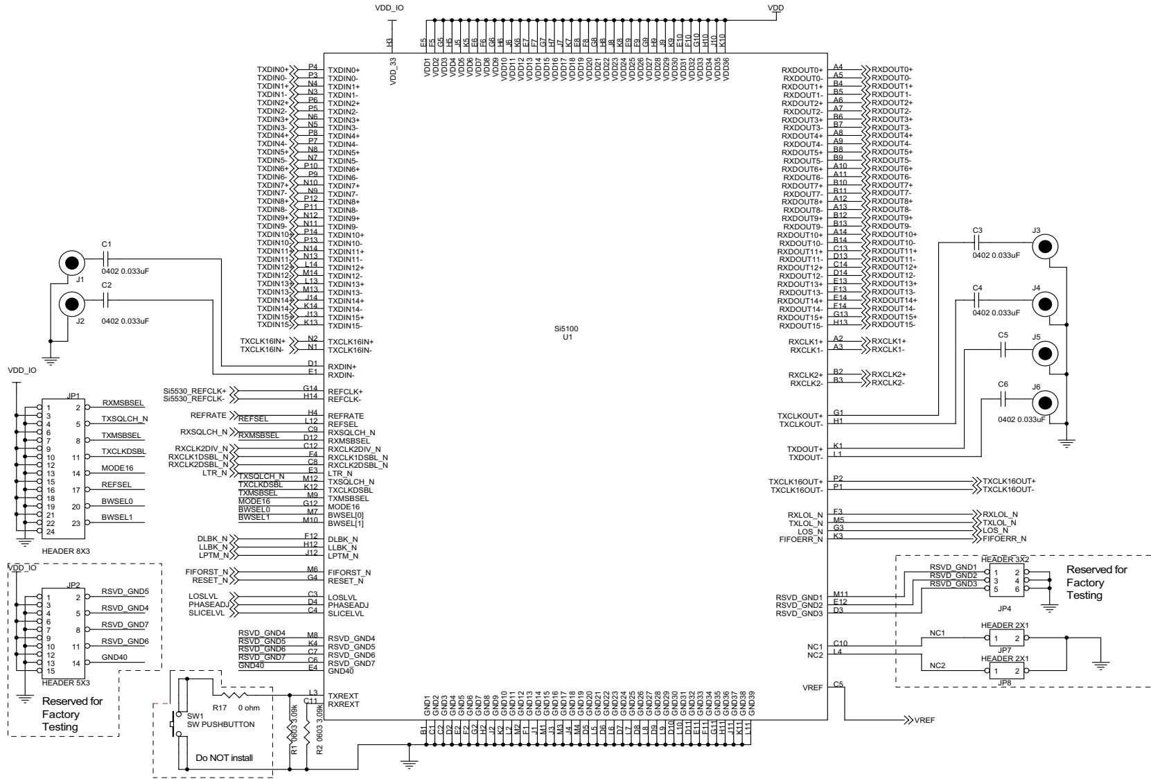
Figure 8. Si5100-EVB Daughter Card Schematic (page 1 of 3)
