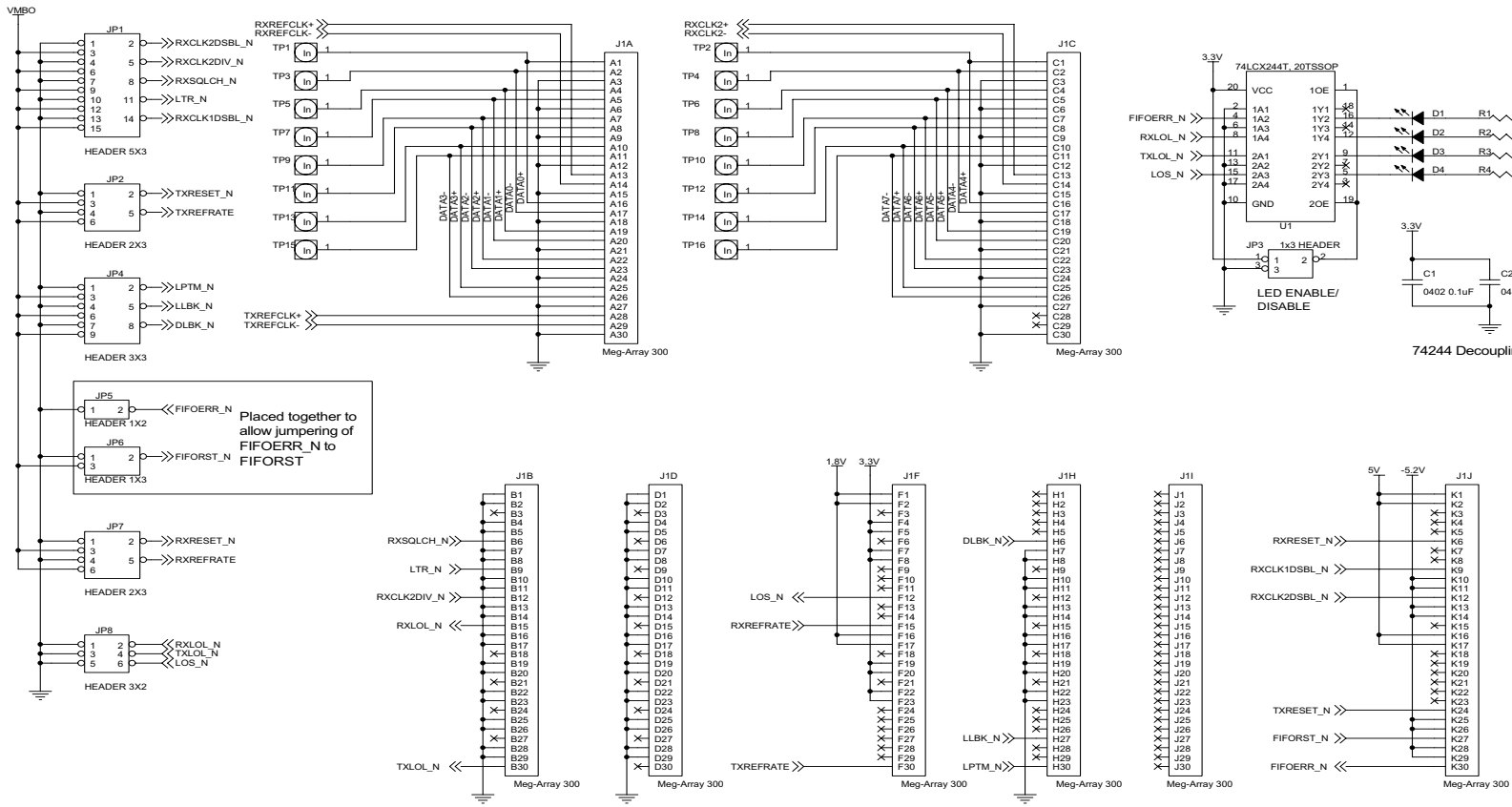
Figure 15. Loopback Motherboard Schematic (page 2 of 2)
