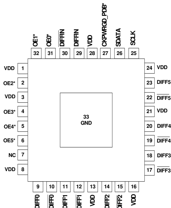
Figure 4. 32-Pin QFN
