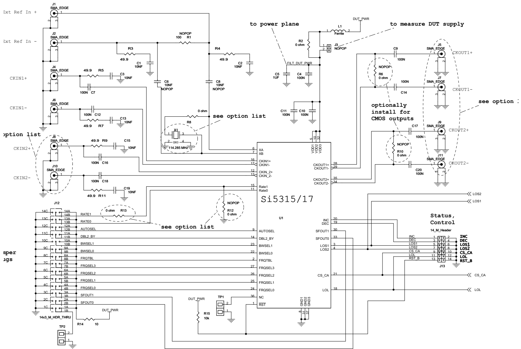
Figure 3. Si5317-EVB
