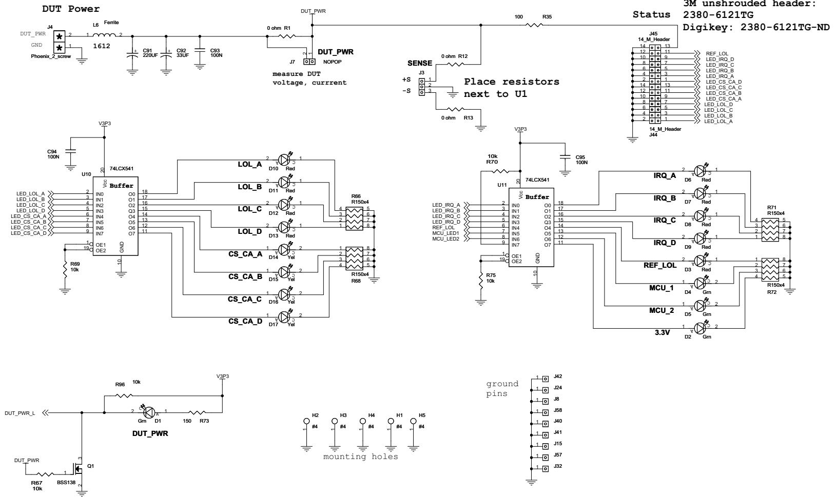
Figure 10. Power and LEDs
