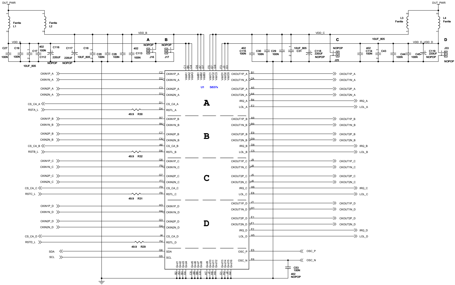
Figure 4. Si537x
