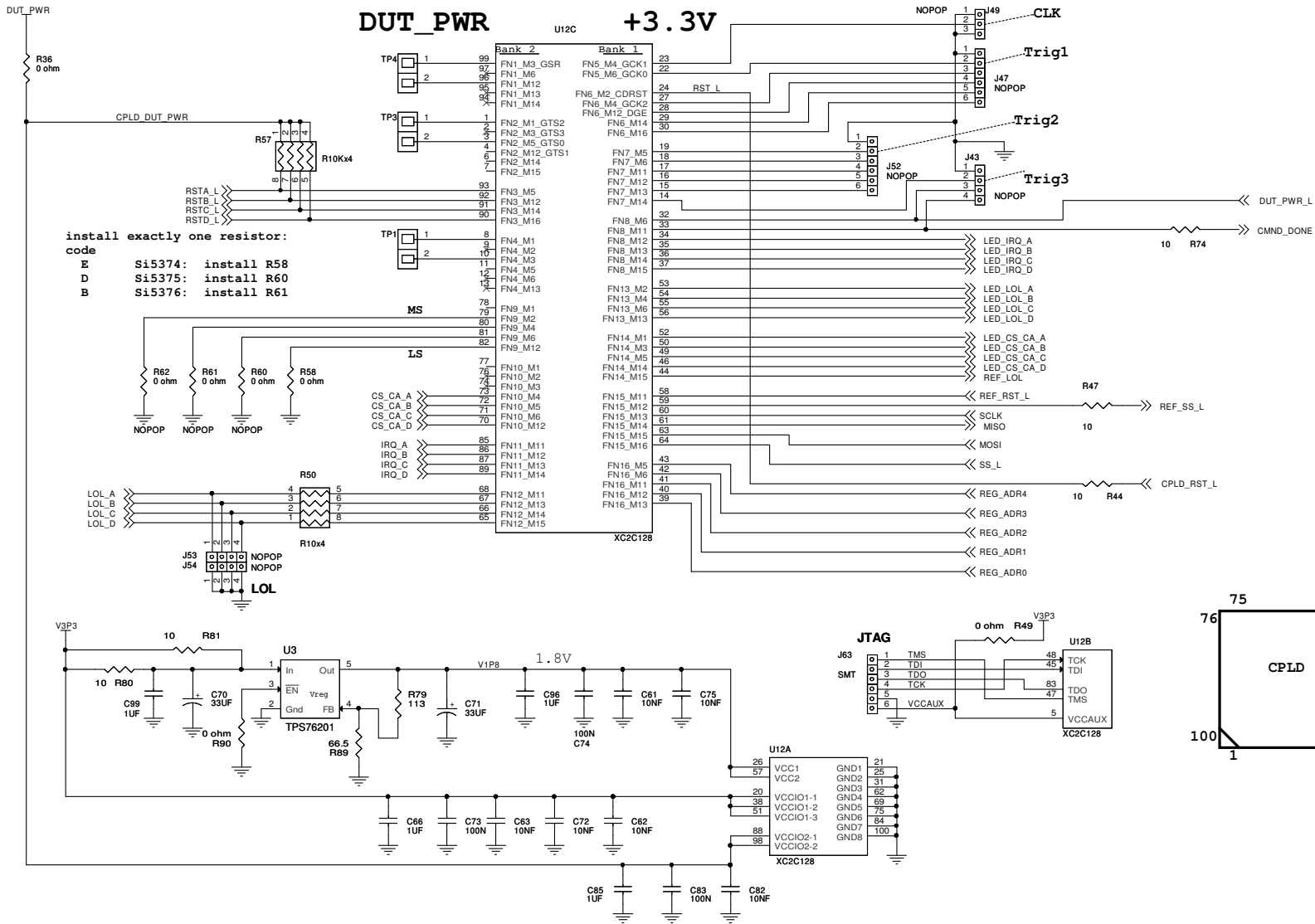
Figure 8. CPLD
