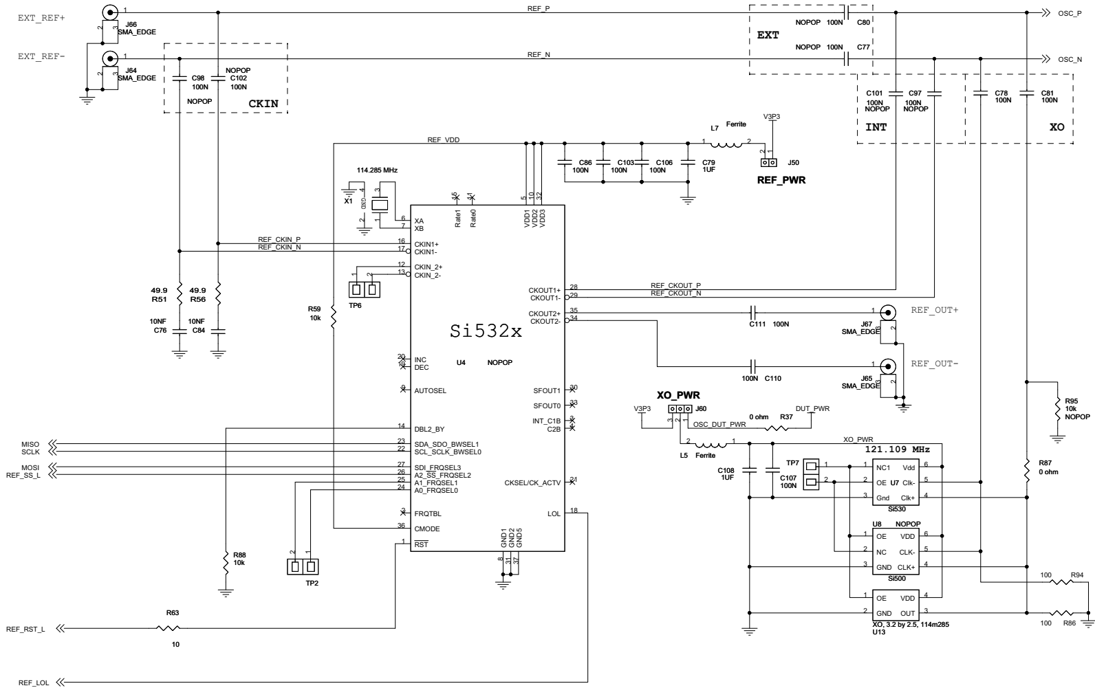
Figure 7. Reference Oscillators
