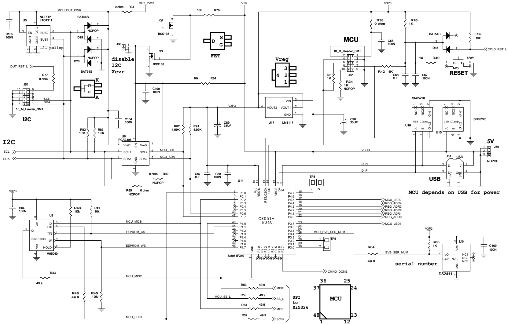
Figure 9. MCU
