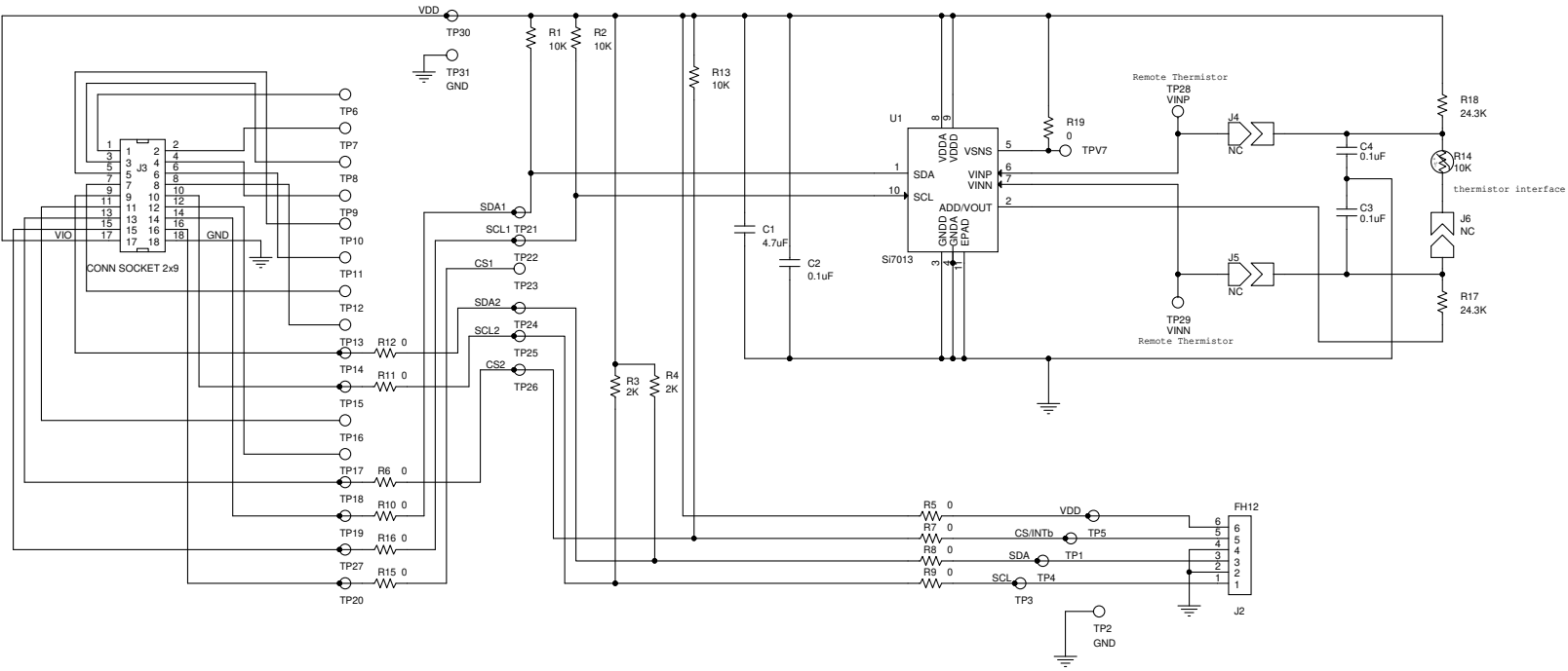
Figure 3. Si7013EB-UDP Schematic
