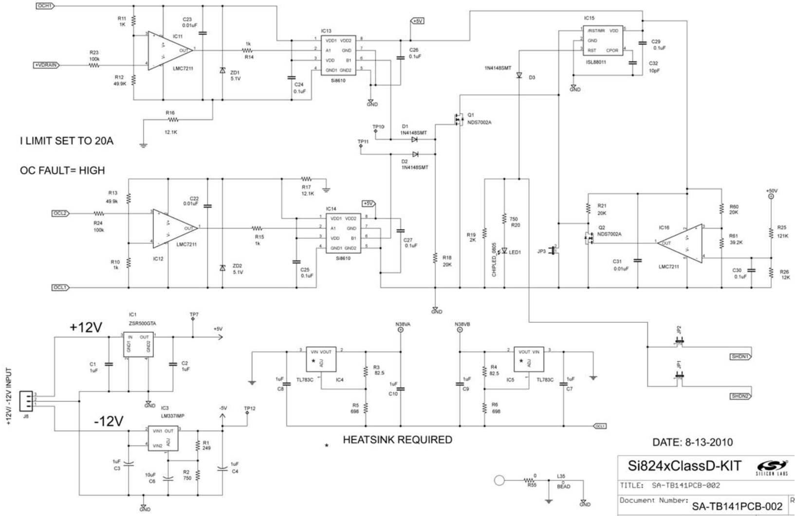
Figure 9. Si824x Class D Audio Amplifier Reference Design Schematic (2 of 2)
