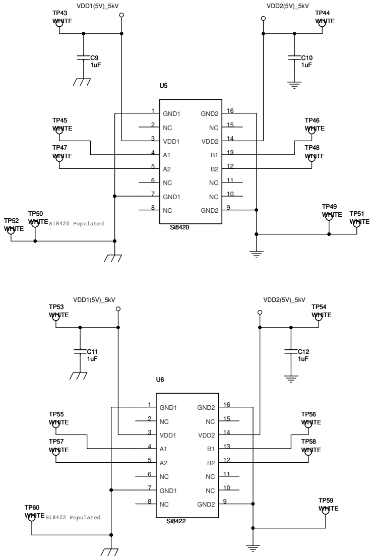
Figure 9. Si84xx5kVISO Evaluation Board Schematic (2 of 2)
