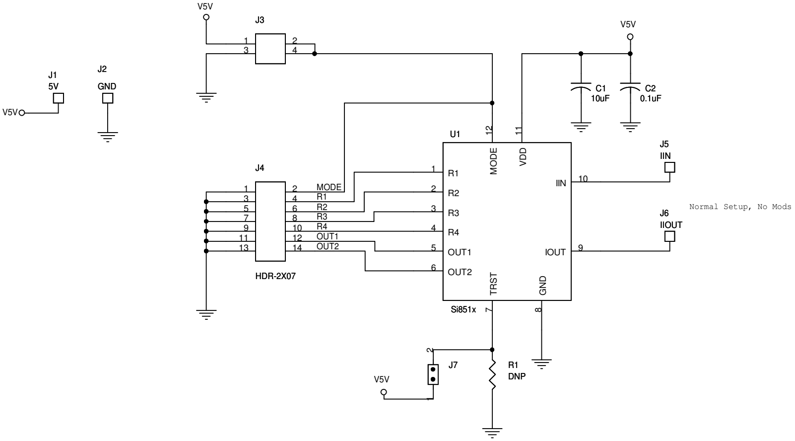
Figure 9. Si85xx-TB Target Board Schematic (1 kV, 10 Amp Target Board)
