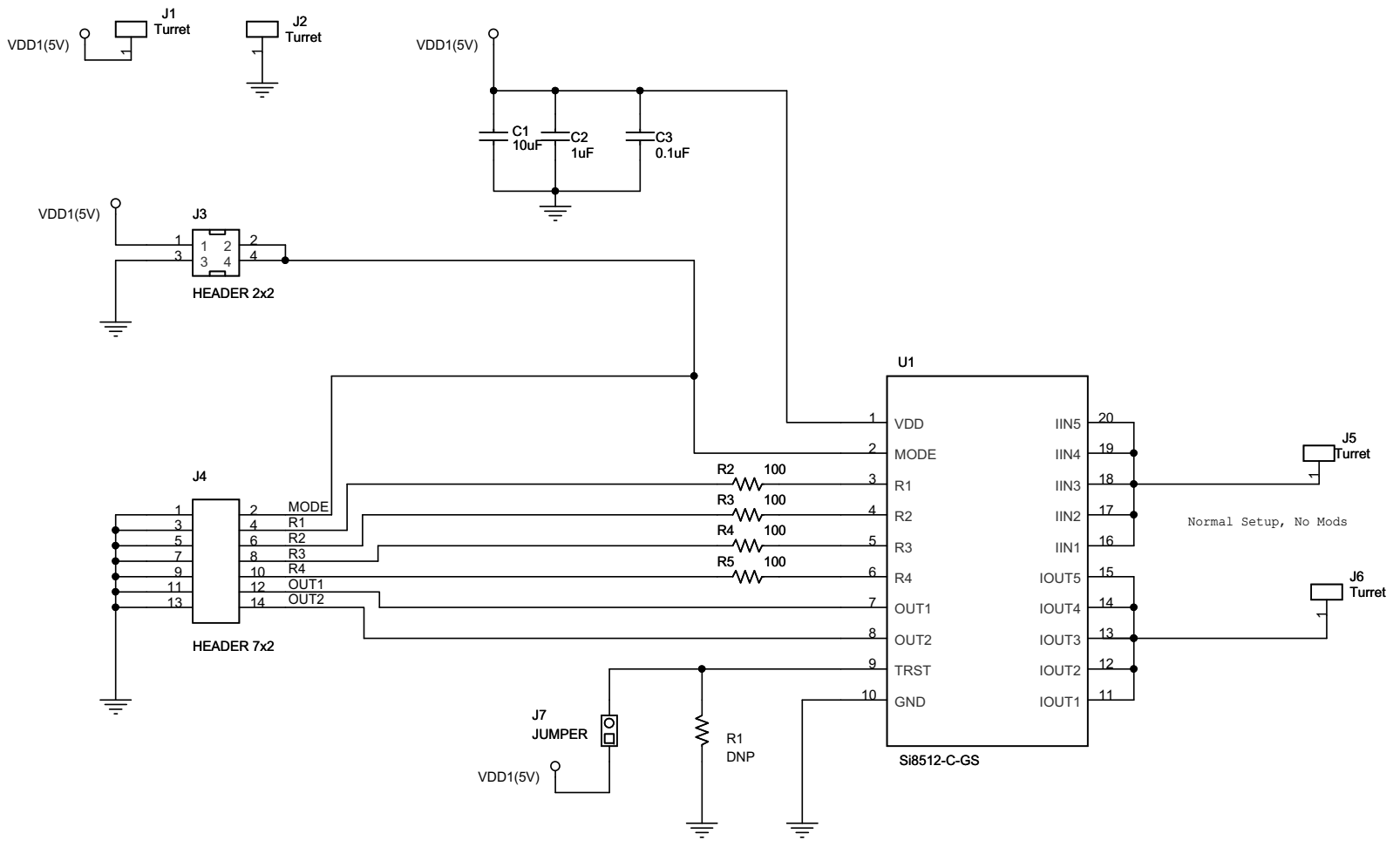
Figure 10. Si85xx5kV-TB Target Board Schematic (5 kV, 10 Amp Target Board)
