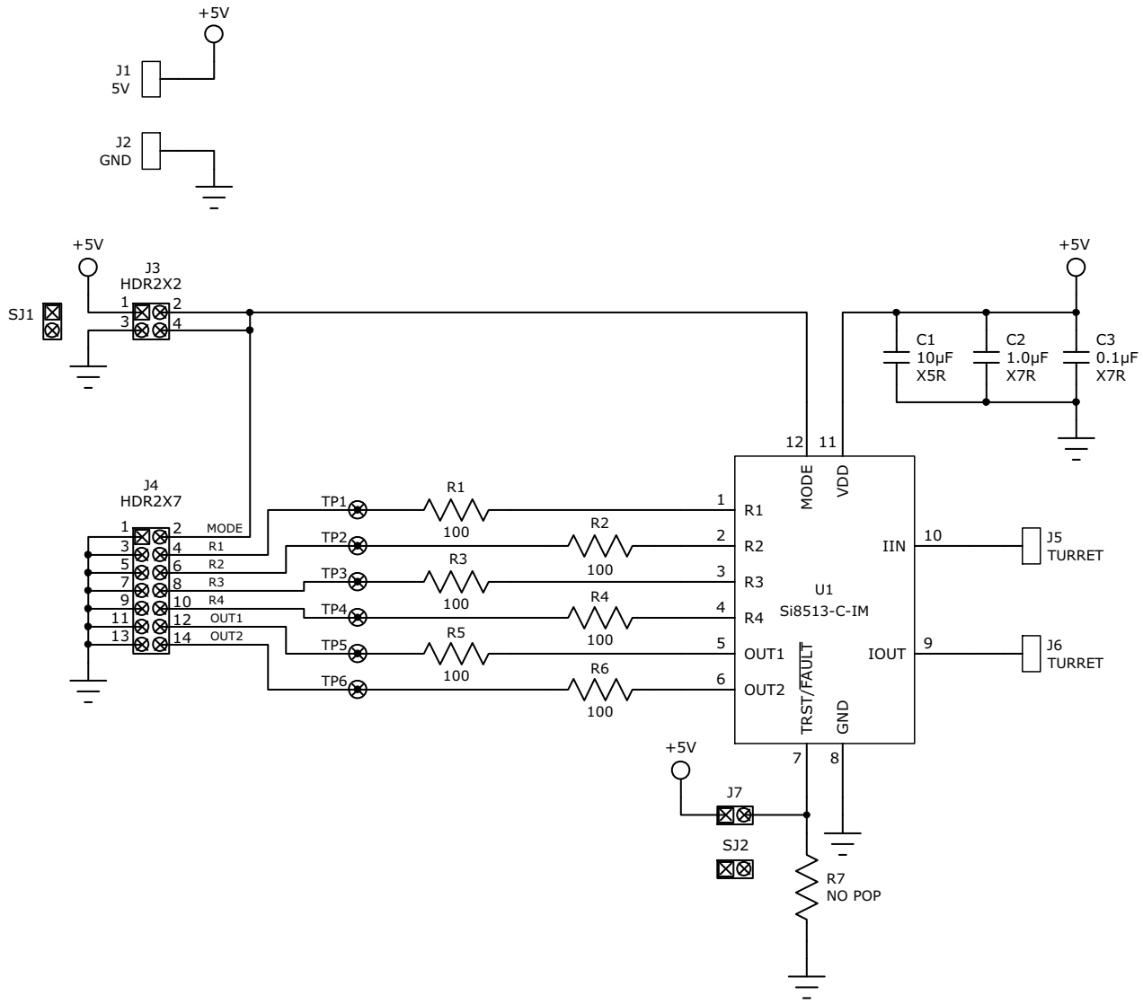
Figure 11. Si85xx20AQFN-TB Target Board Schematic (1 kV, 20 Amp Target Board)
