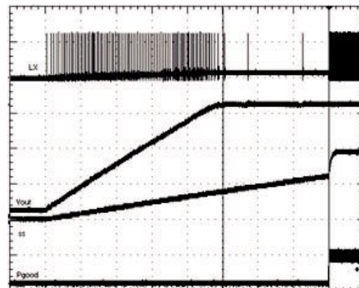
Figure 31 - Soft-Start Timing Diagram
