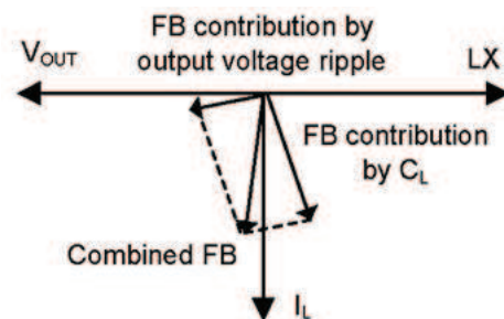
Fig. 17 - FB Voltage in Phasor Diagram
