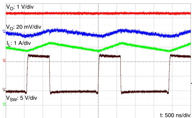
V O ripple and V SW switching waveform. V IN = 12 V, V O = 3.3 V and L = 10 μH (IHL2525EZ type). C O consists of MLCC of 4.7 μF and tantalum of 100 μF/20 V x 2
