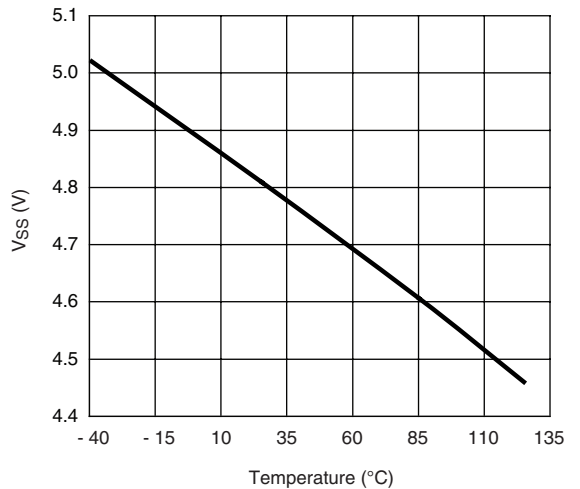
V_{SS} vs. Temperature
