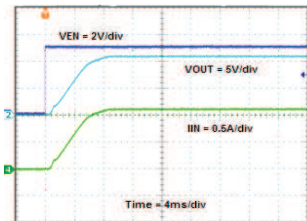
Fig. 23 - Turn-ON Time, V_{IN} = 12\text{ V} , C_{SS} = 47\text{ nF} , R_L = 10\ \Omega , C_L = 10\ \mu\text{F}
