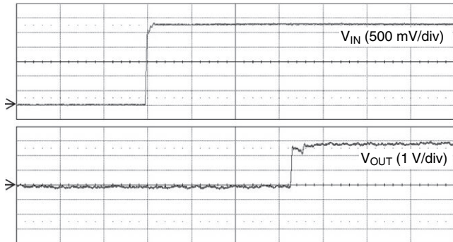
200 ns/div V_{IN} = 2.8 \text{ V} , R_{LOAD} = 18 \Omega , L_{LOAD} = 80 \mu\text{H} Input Rising Edge Trigger Response Time
