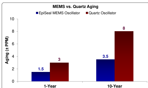
Figure 2. Aging Comparison [2]
