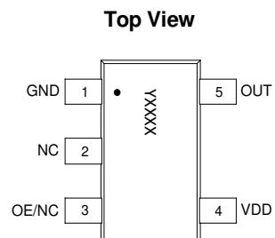
Figure 1. Pin Assignments
