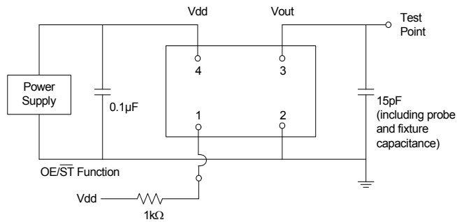
Figure 1. Test Circuit
